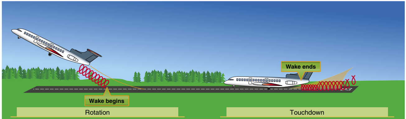
Figure 13-21. Vortex behavior.
