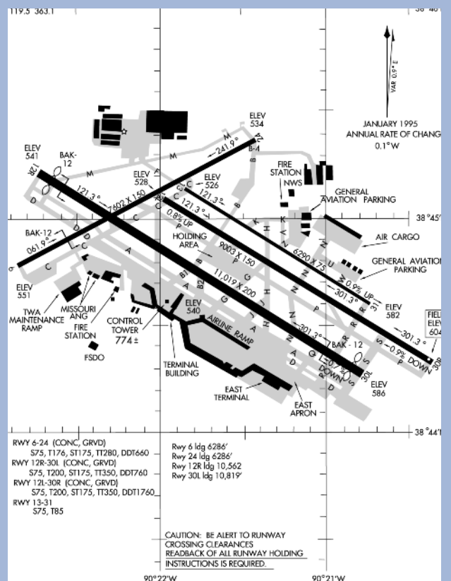
AIRPORT DIAGRAM
