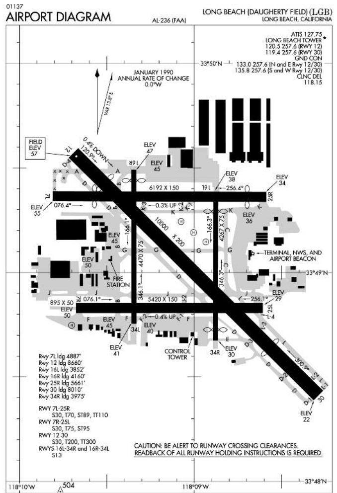
AIRPORT DIAGRAM LONG BEACH (DAUGHERTY FIELD) (LGB) 01137
