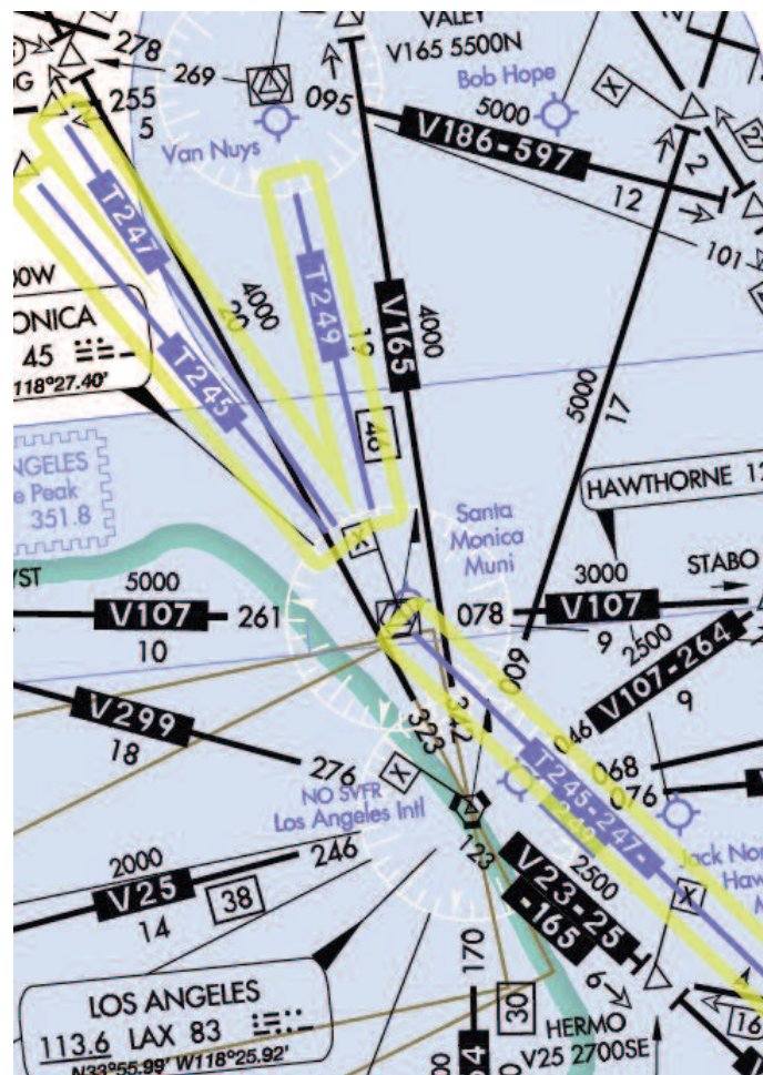
Figure 10. RNAV IFR Terminal Transition Routes
