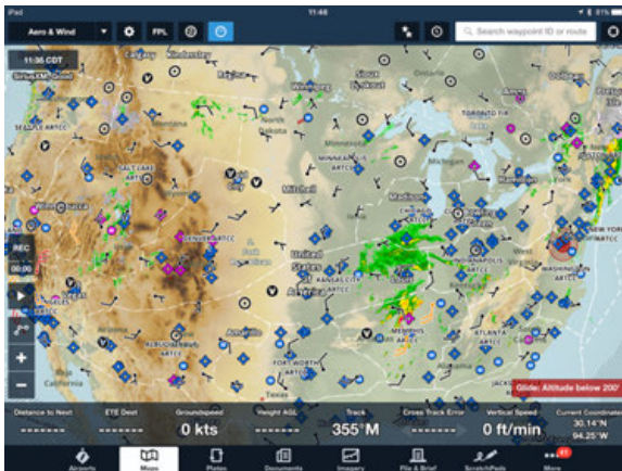
Surface Winds
